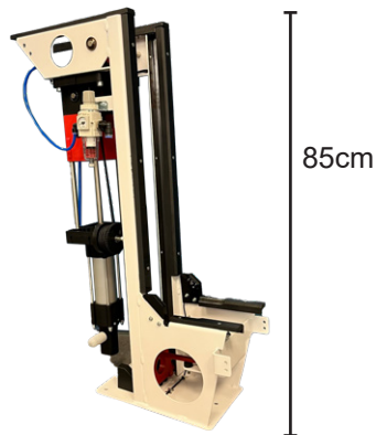
airOlift 85cm (front of bowling lane) 531103
