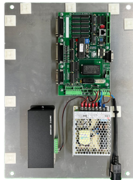
Control baseplate with power supply & RGBW controller 551112
