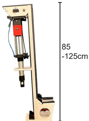
airOvator 85 or 125cm (machine side) 531102
