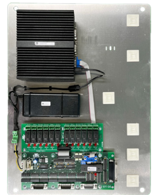
Lane scoring baseplate with scoring computer & I/O interface boards 551122
