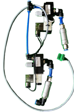
Bumper valves incl. check valves complete assembled 541143
