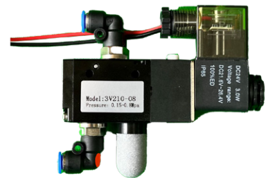
Electrical pneumatic valve for airOlift & air- Ovator (pre-assembled) 541141
