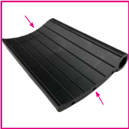
Bumper flip part (holes on both sides) 531127
