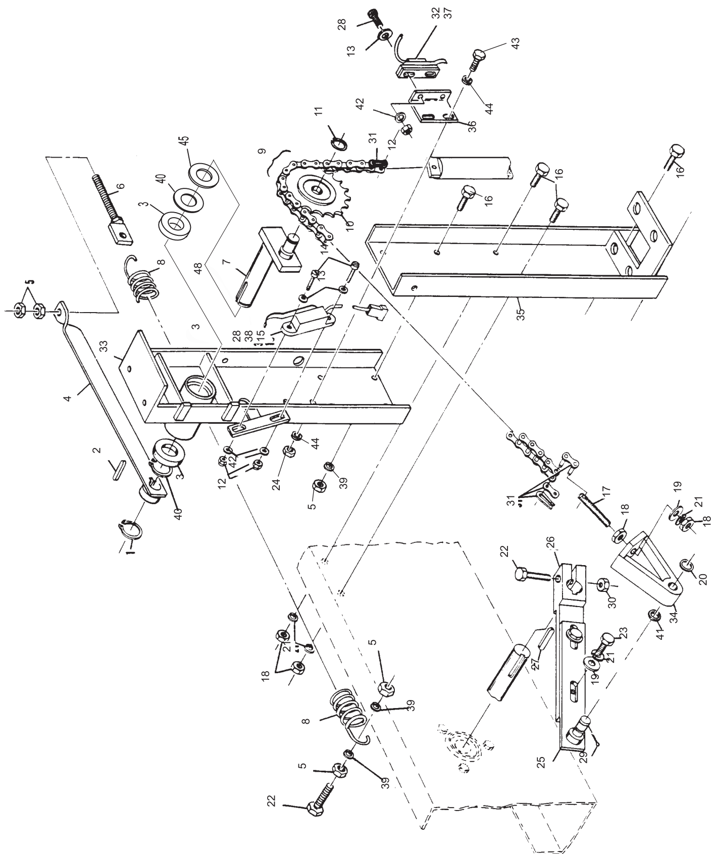
Two Piece Guide Tower Assembly
