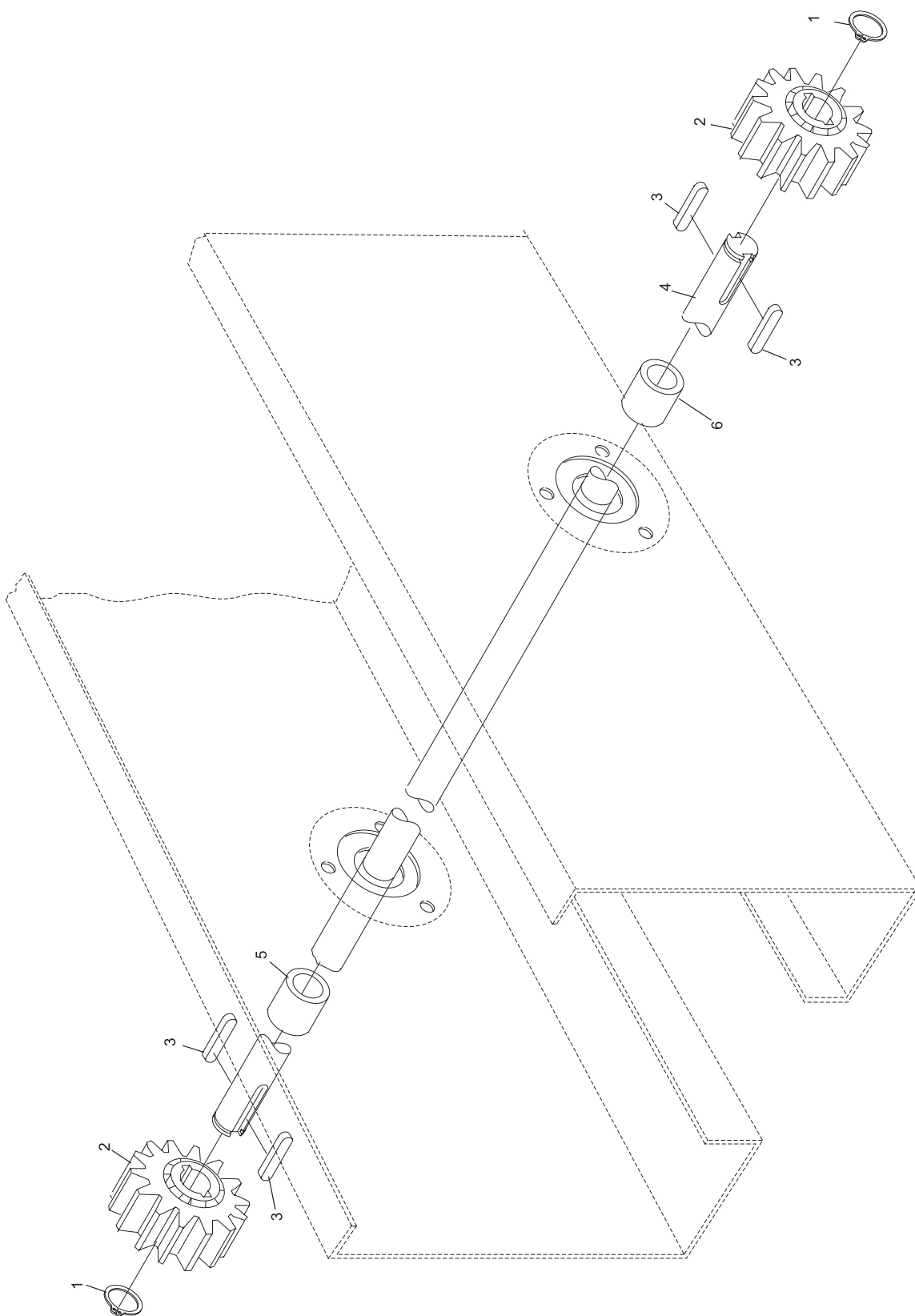
Setting Table Pinion Shaft Assembly
