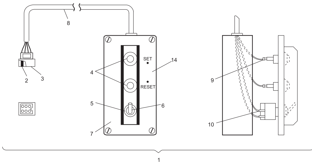
Rear Control Box Cable Assembly
